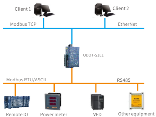
Typical application topology
