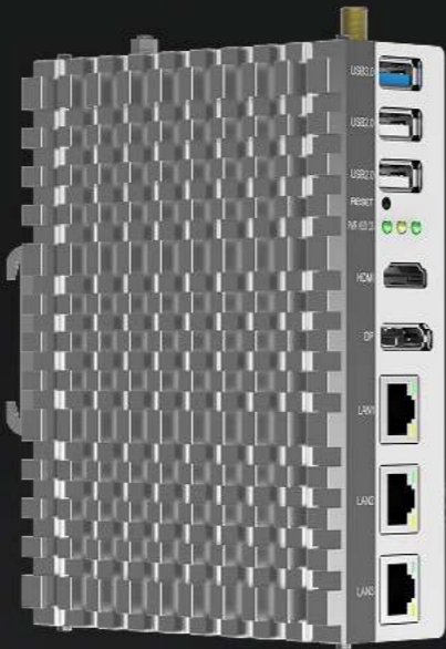
PC6012 Intel® Celeron® J6412 3 x RJ45 1 x DP + 1 x HDMI 3 x USB
