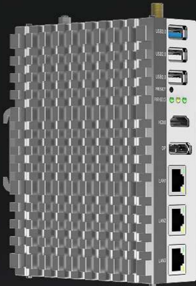
PC6010 Intel® Celeron® J1900 3 x RJ45 1 x DP + 1 x HDMI 3 x USB
