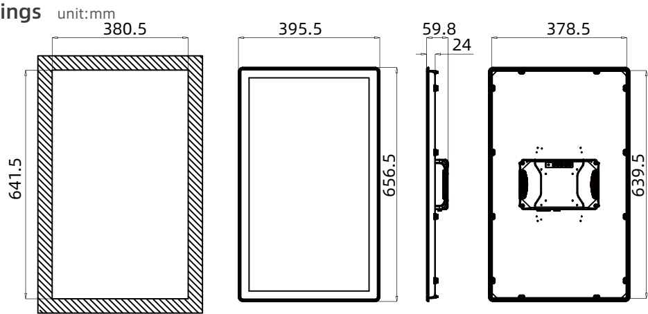
Panel Cutout Dimensions: 380.5 x 641.5mm ( 14.98 x 25.26in )
